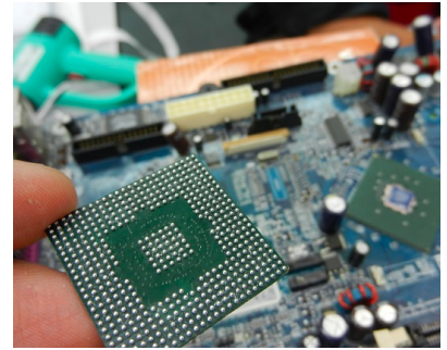
BGA Rework
