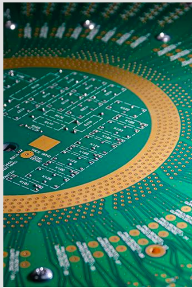
Probe Card
